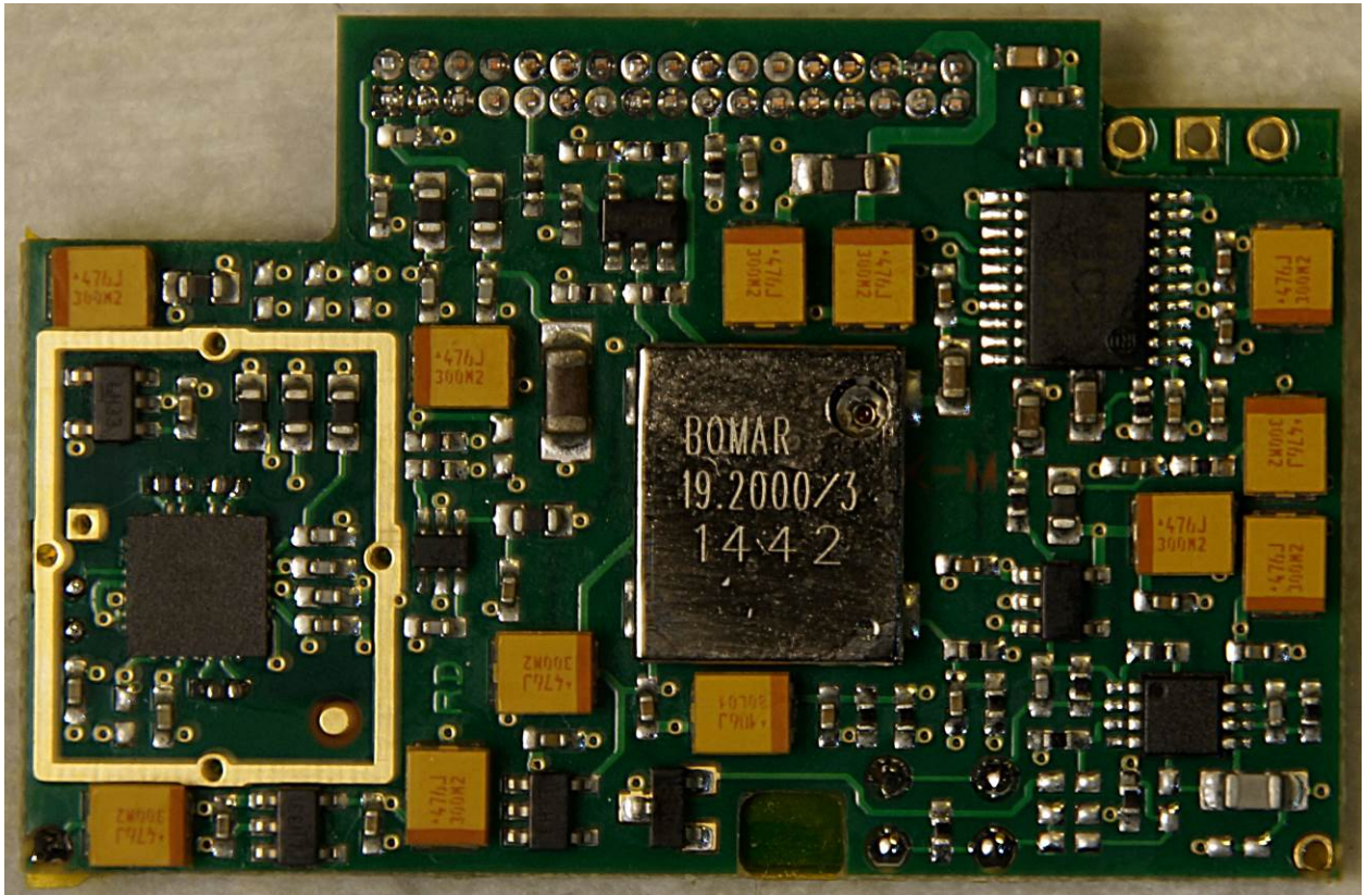
Figure 2: Audio Board – Top View Without Shielding
