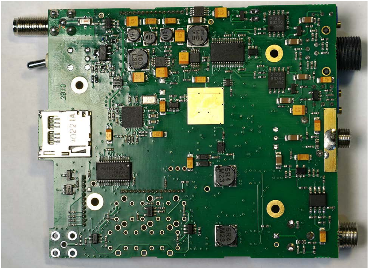
Figure 6: Main Board – Bottom View
