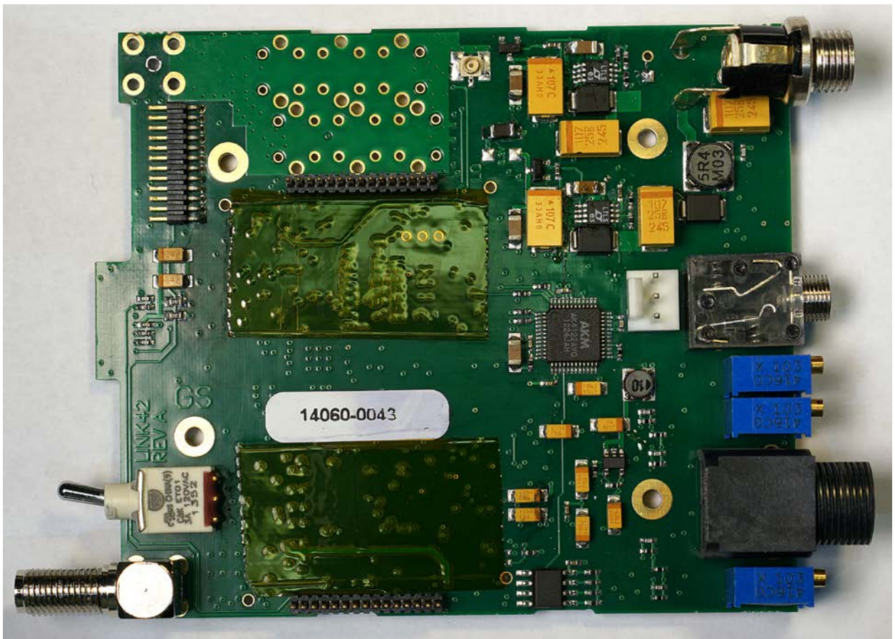
Figure 5: Main Board – Top View
