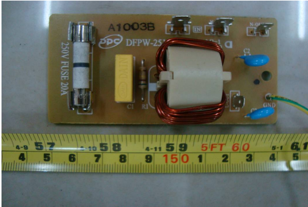
EUT – Filter Board Top View
