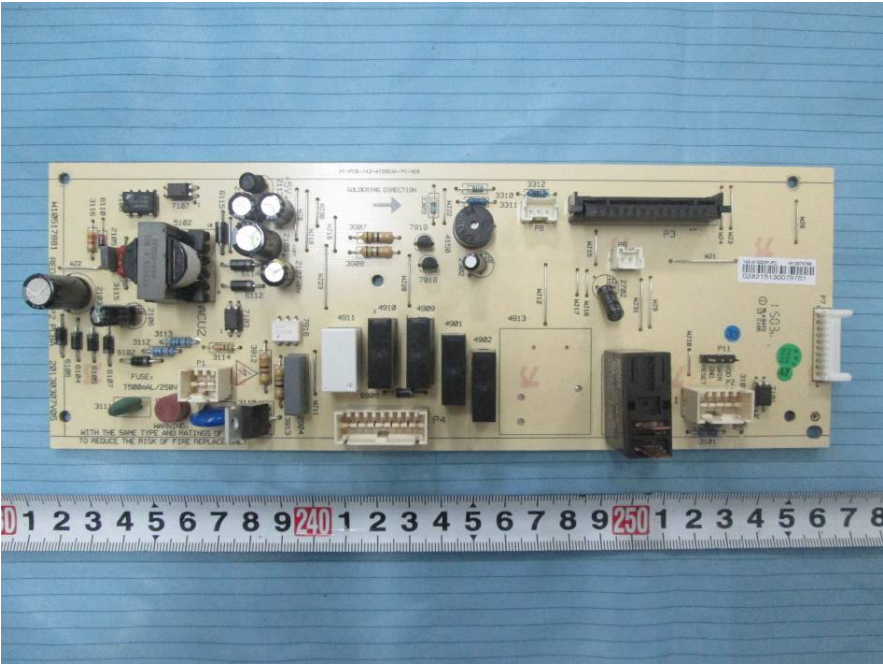
EUT – Control Panel PCB Top View
