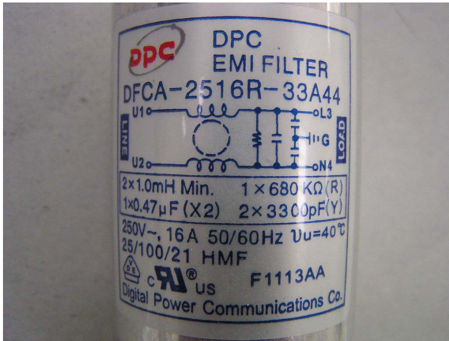
EUT-Cap View
