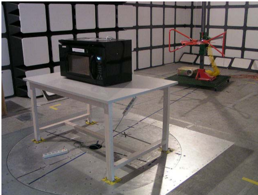
30 MHz to 1000MHz: Radiated Emissions-Front View
