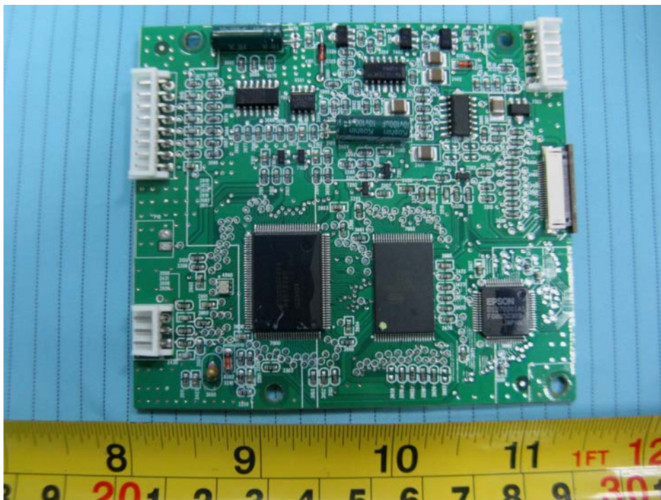
EUT – Operation Control Board Top View
