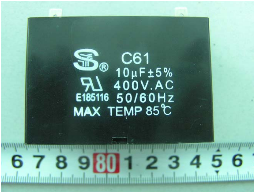
EUT- High Capacitor View
