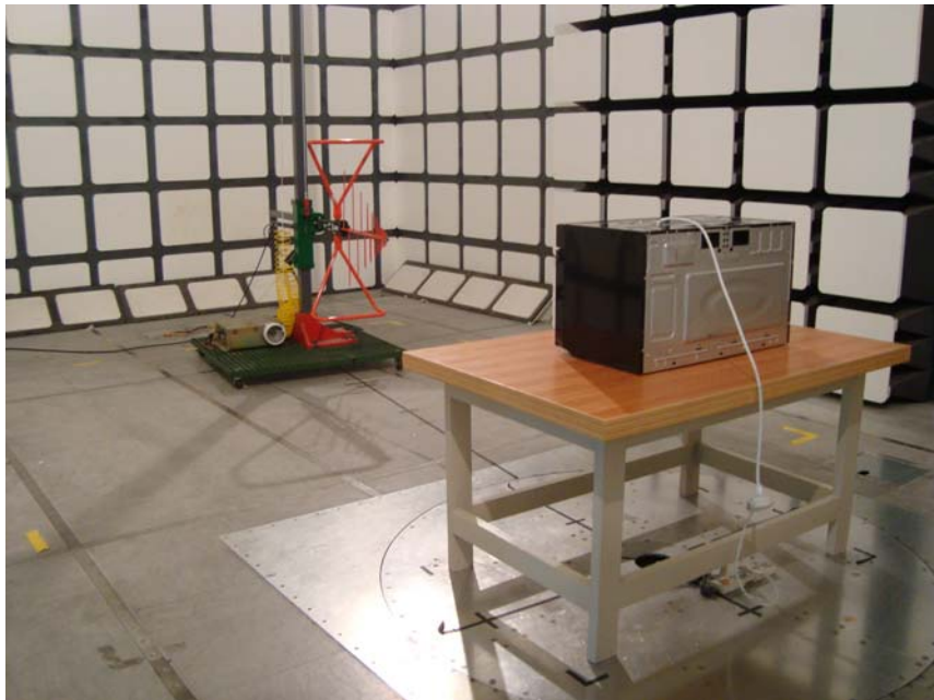
Radiated Emissions - Rear View (30 MHz-1 GHz)
