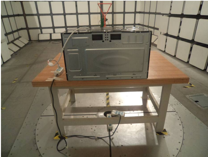
Radiated Emissions (30 MHz to 1GHz) - Rear View
