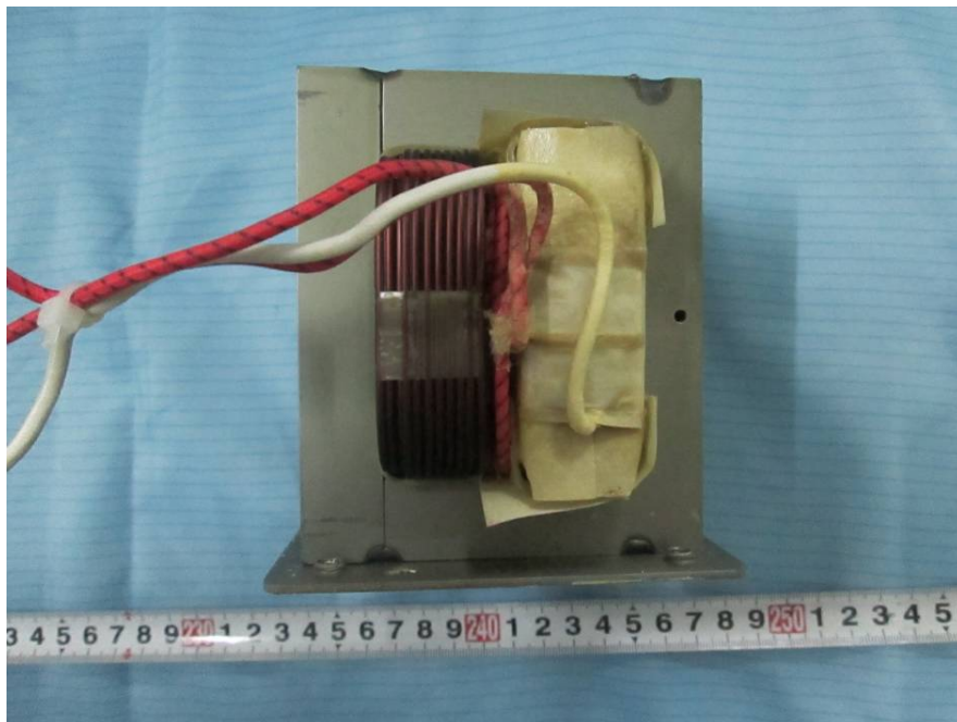
EUT – Power Transformer Rear View
