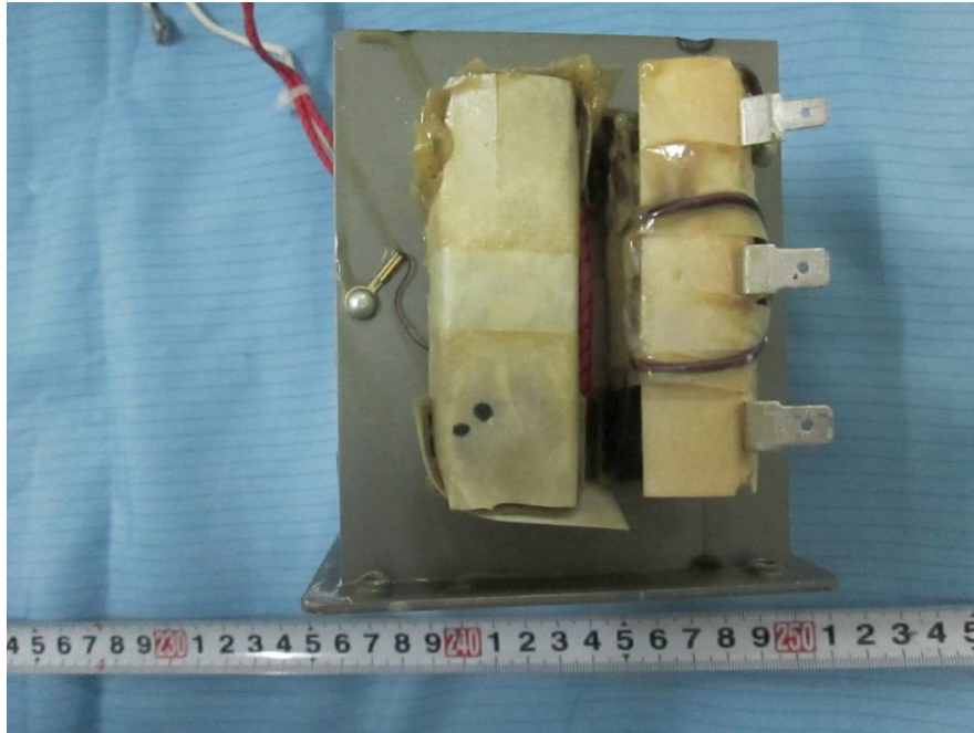
EUT – Power Transformer Front View
