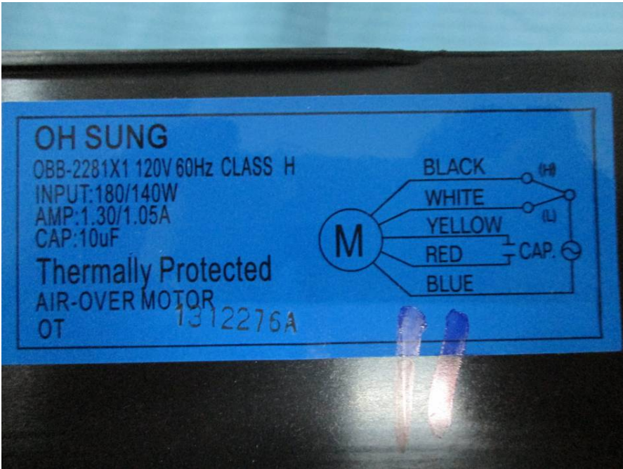
EUT – Air-Over Motor Label View
