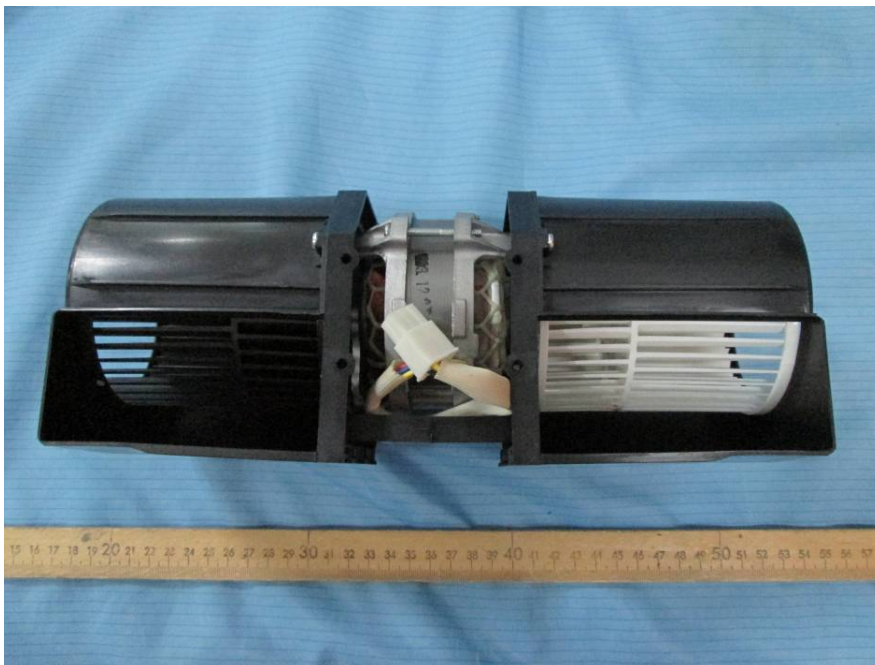
EUT – Air-Over Motor View
