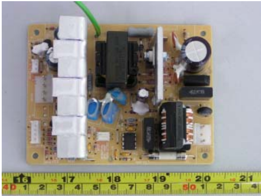
EUT – DC Transformer PCB Top View
