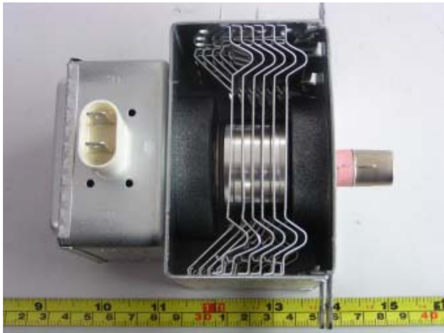
EUT – Magnetism Signal Generator Side View
