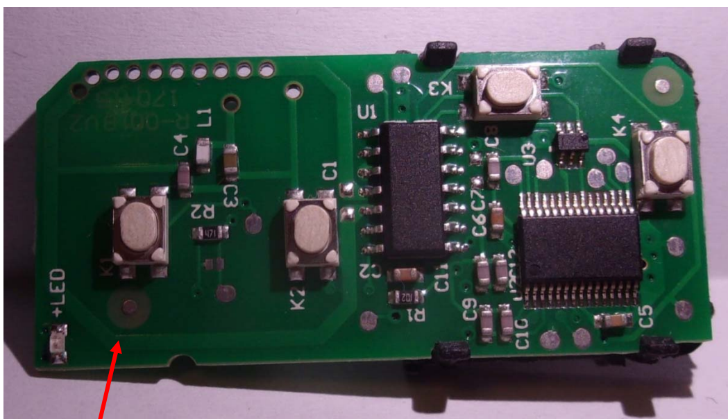
PCB Antenna
