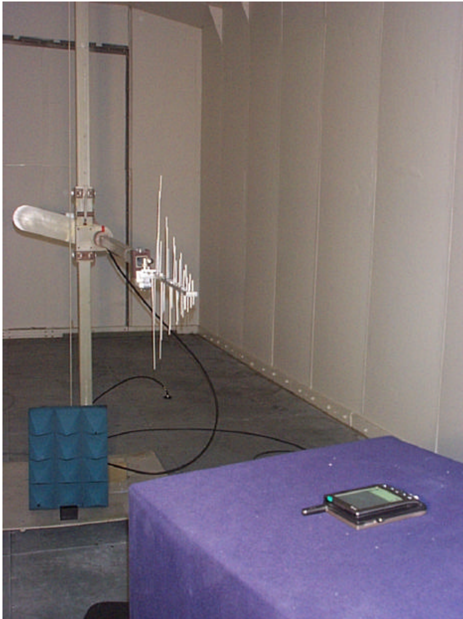
ERP Testing – Horizontal Position
