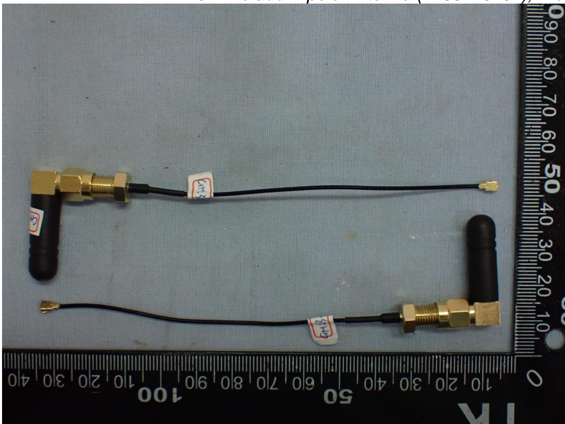
Figure 10 This Time add Dipole Antenna (2158720101), Front View
