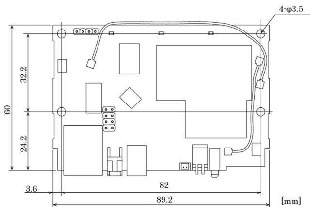
Figure 8.1. External Dimensions
