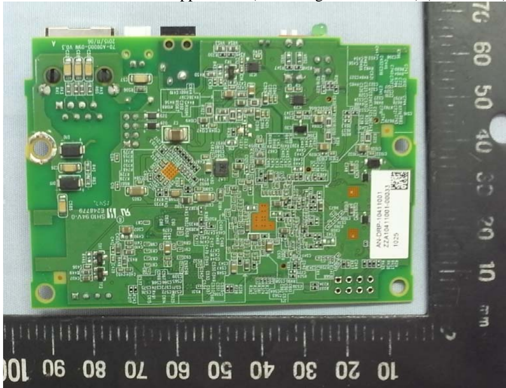
Figure 4 General Appearance (with Integrated Antenna) (Back View)
