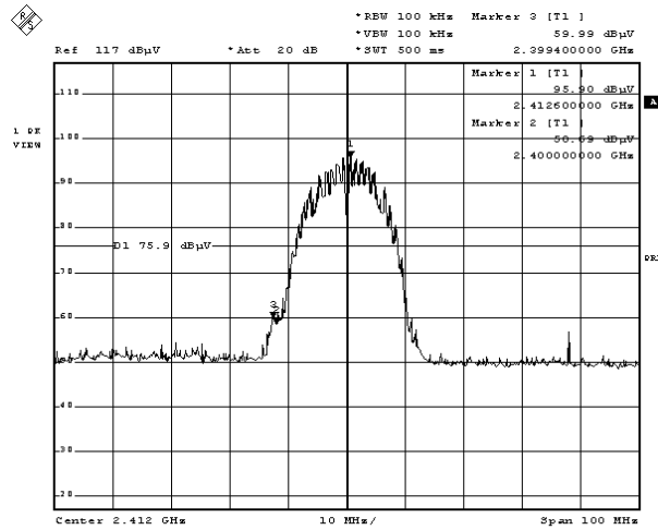
Figure Channel 1: (Horizontal)
