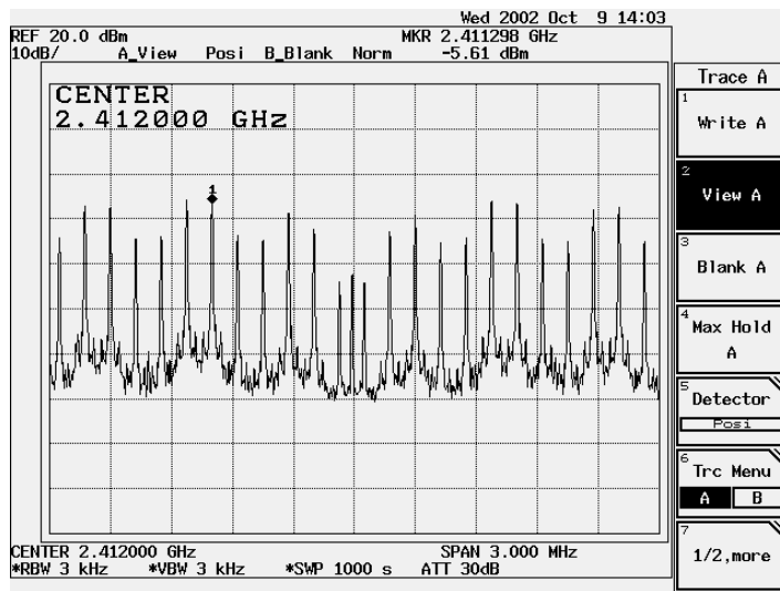
Figure Channel 1: 11Mbps
