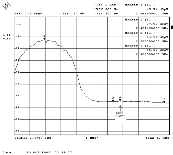
Figure Channel 11: (Horizontal)
