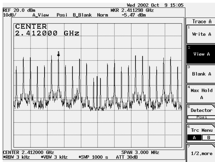
Figure Channel 1: 11Mbps
