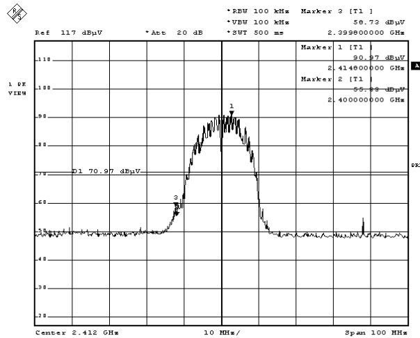
Figure Channel 1: (Vertical)
