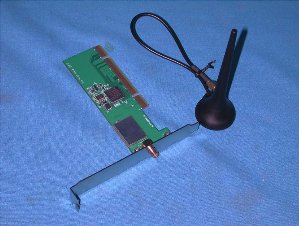
(1) EUT Photo
