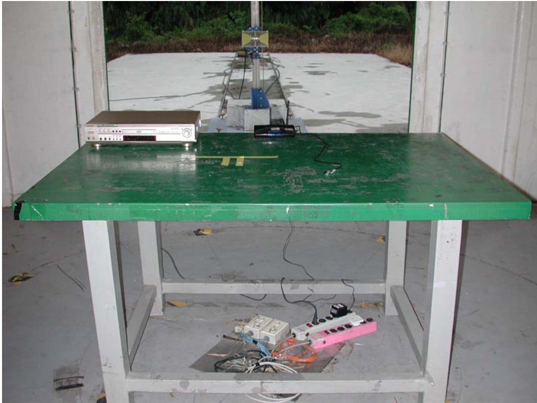
Back View of Radiated Test (High Frequency)
