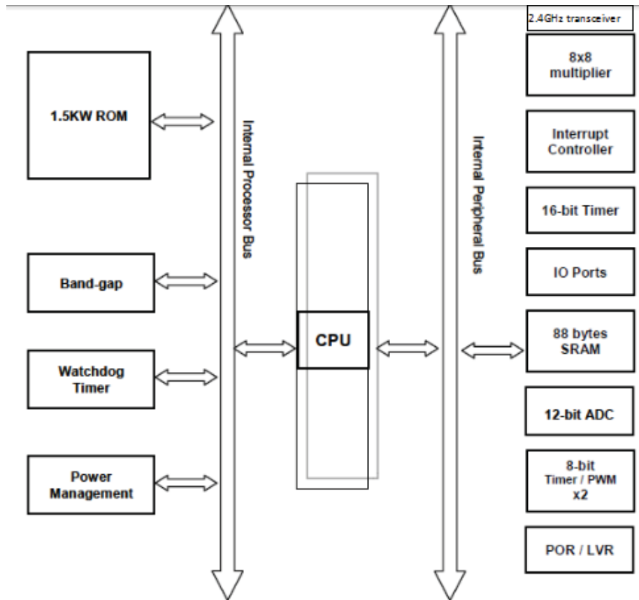
Chart1 FW1210 SOC block diagram
