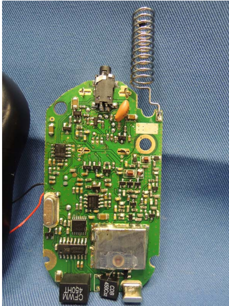
Main PCB View 1
