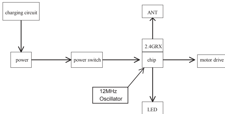
66807RXV4A- block diagram
