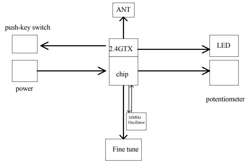
ABE2402X1-66804TXV1-block diagram
