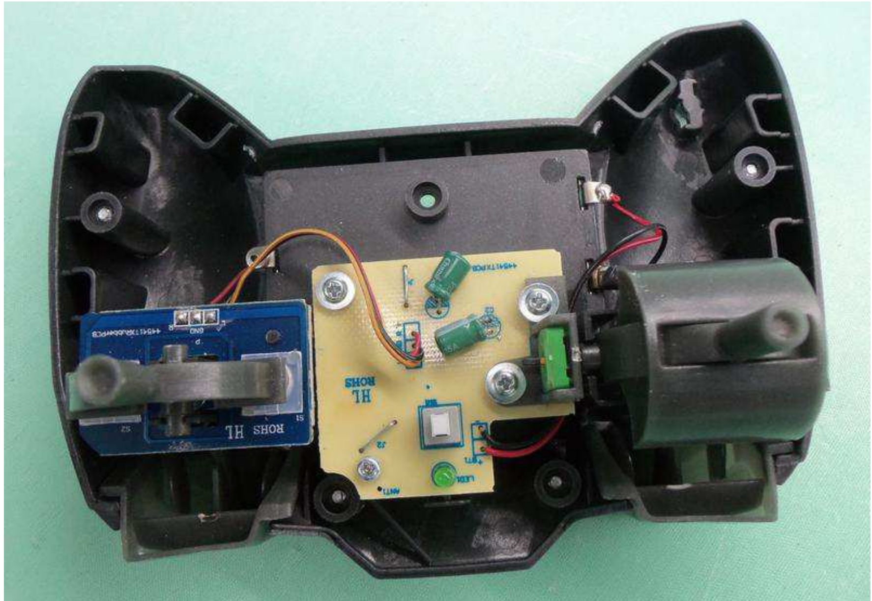
FCC ID: PQN44541TX2G4 PHOTOGRAPH OF THE PRODUCT
