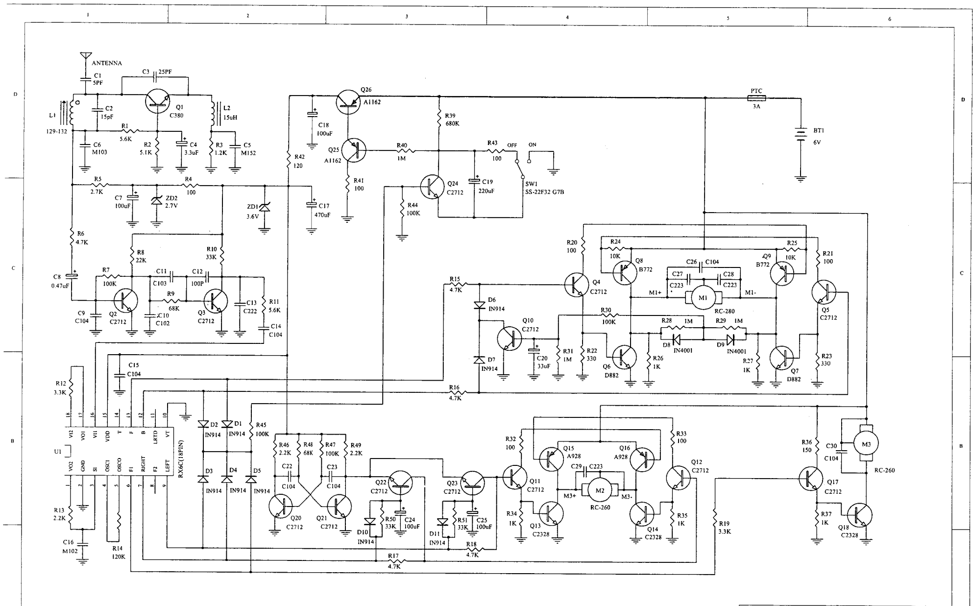
HERALD METAL & PLASTIC WORKS LTD. SPIN MASTER #40155 (49MHZ) RECEIVER CIRCUIT DIAGRAM
