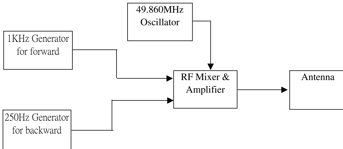
Wiggle RC Car 49.860MHz Tx Block Diagram
