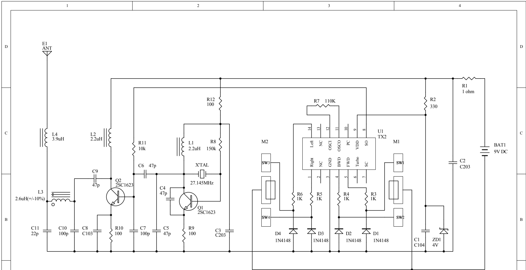
SPIN MASTER #14127 Wall Racer - Transmitter (27.145MHz) Circuit Diagram
