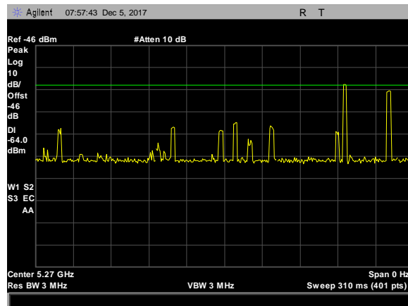
Plot 14. Radar Waveform Calibration, 5270 MHz, Type 6, 40 MHz
