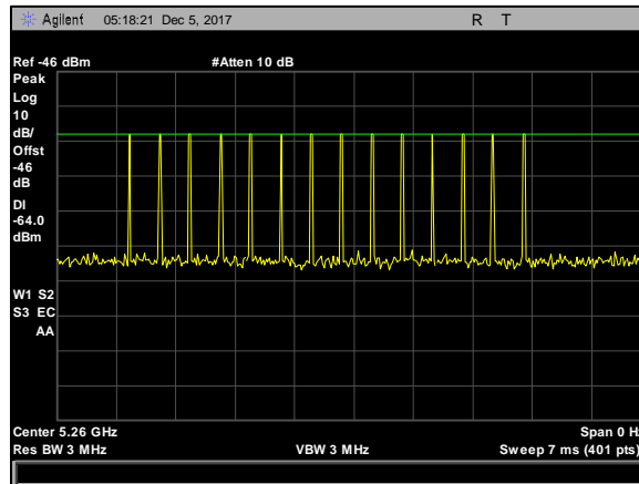
Plot 5. Radar Waveform Calibration, 5260 MHz, Type 4, 20 MHz
