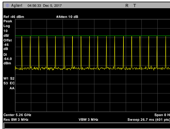
Plot 1. Radar Waveform Calibration, 5260 MHz, Type 0, 20 MHz
