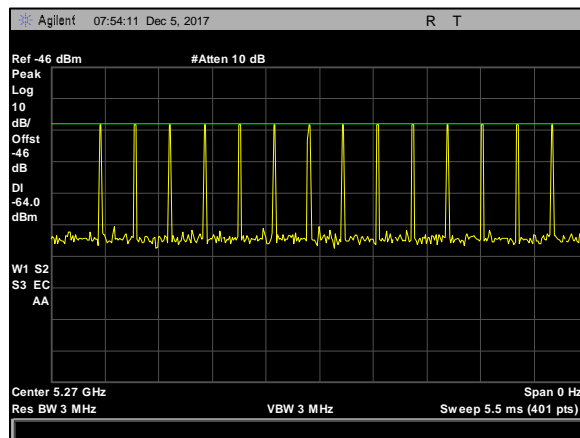
Plot 12. Radar Waveform Calibration, 5270 MHz, Type 4, 40 MHz
