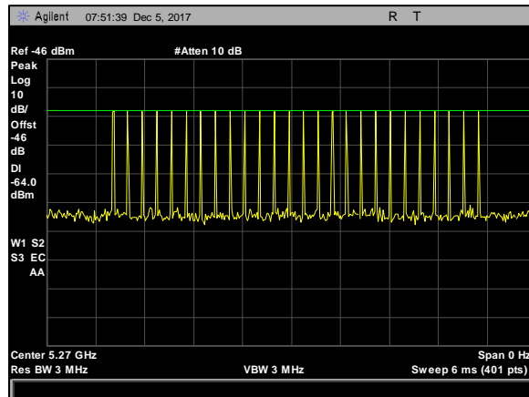
Plot 10. Radar Waveform Calibration, 5270 MHz, Type 2, 40 MHz
