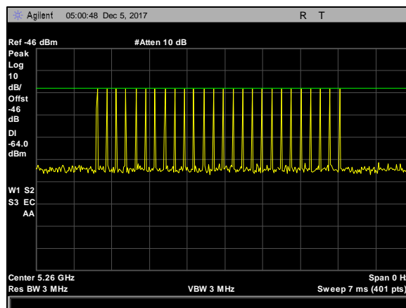
Plot 3. Radar Waveform Calibration, 5260 MHz, Type 2, 20 MHz
