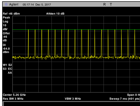
Plot 4. Radar Waveform Calibration, 5260 MHz, Type 3, 20 MHz
