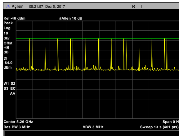
Plot 6. Radar Waveform Calibration, 5260 MHz, Type 5, 20 MHz
