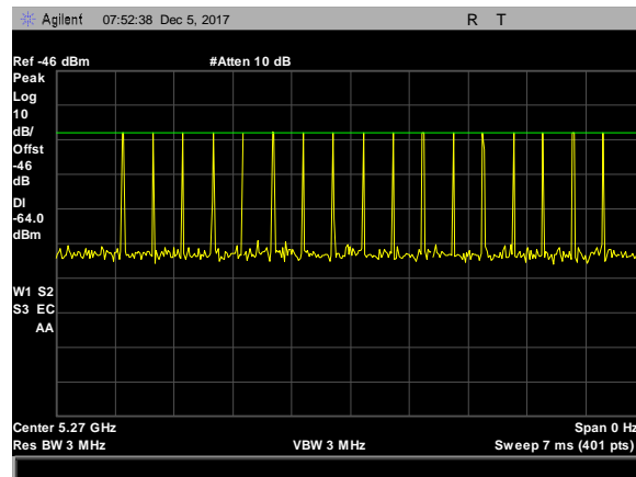
Plot 11. Radar Waveform Calibration, 5270 MHz, Type 3, 40 MHz
