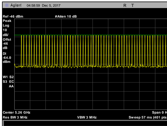
Plot 2. Radar Waveform Calibration, 5260 MHz, Type 1, 20 MHz
