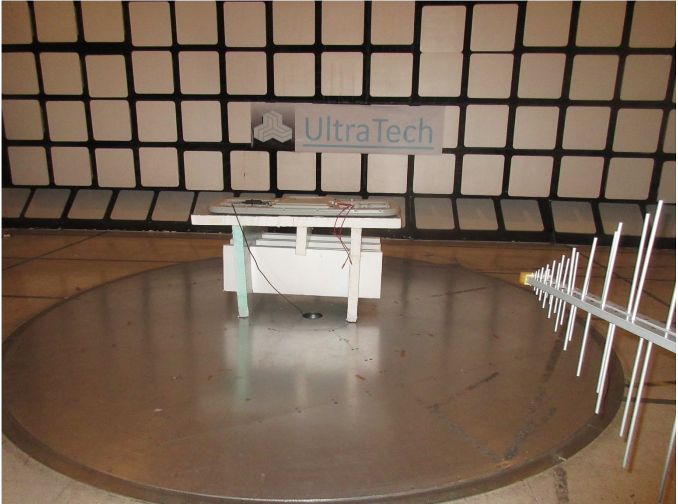
Radiated Emissions at 3 m, 30 – 1000 MHz
