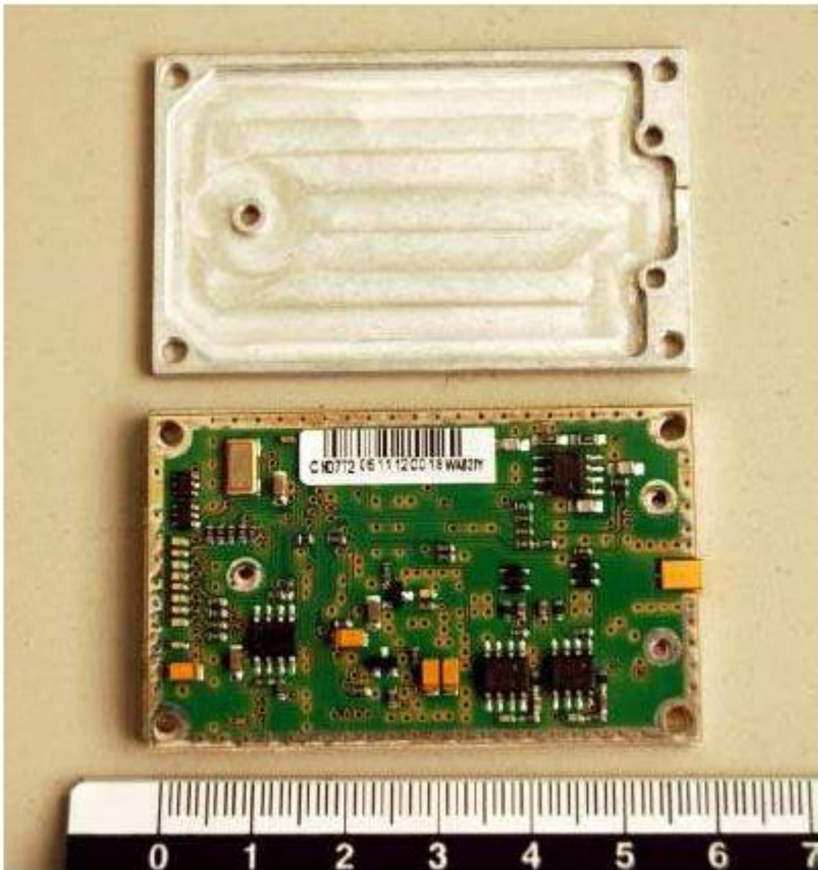
Figure 3: Front of chip
