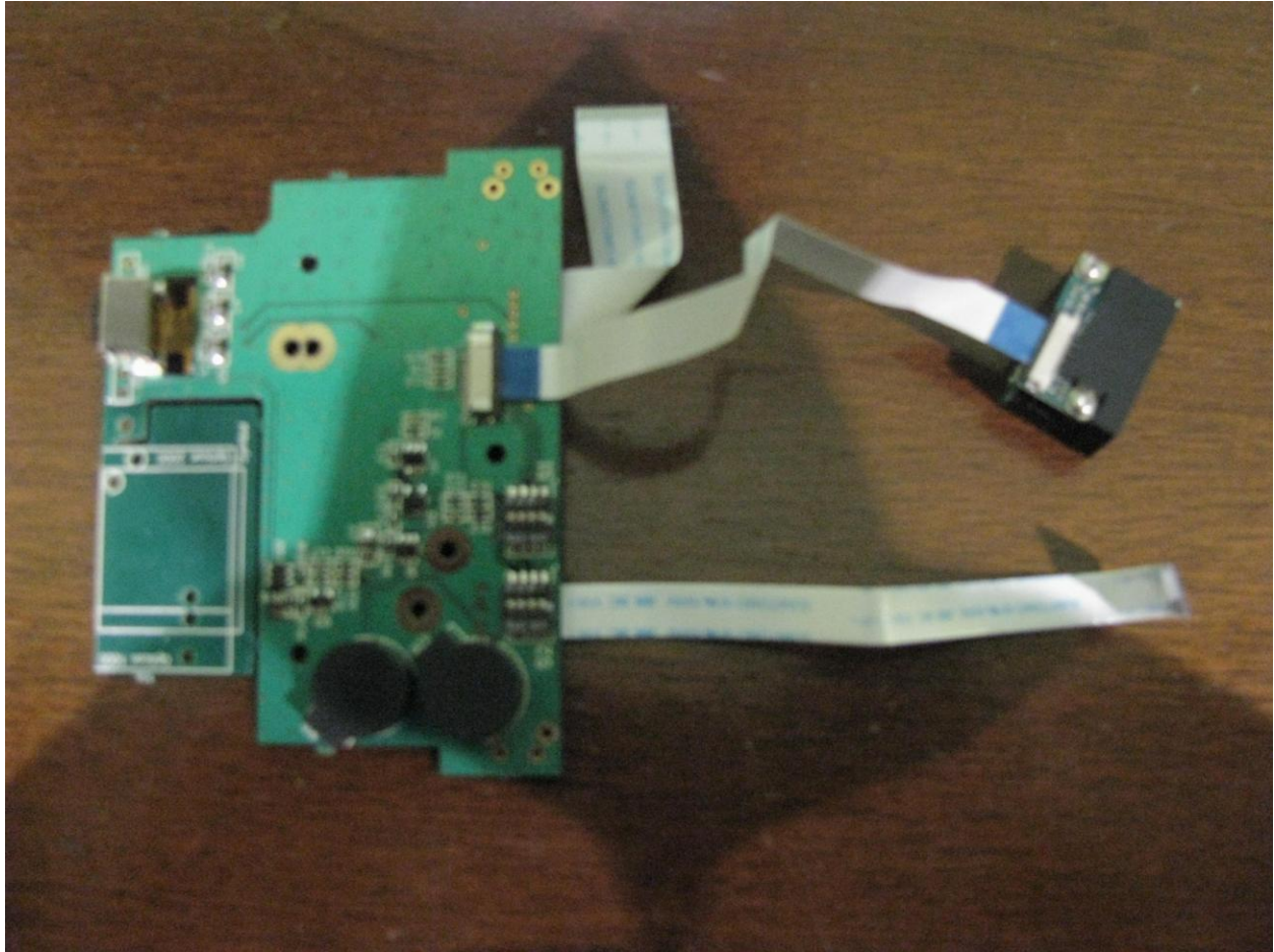
Figure 8: IR Port PCB (Placed on top cover of EUT) Top side
