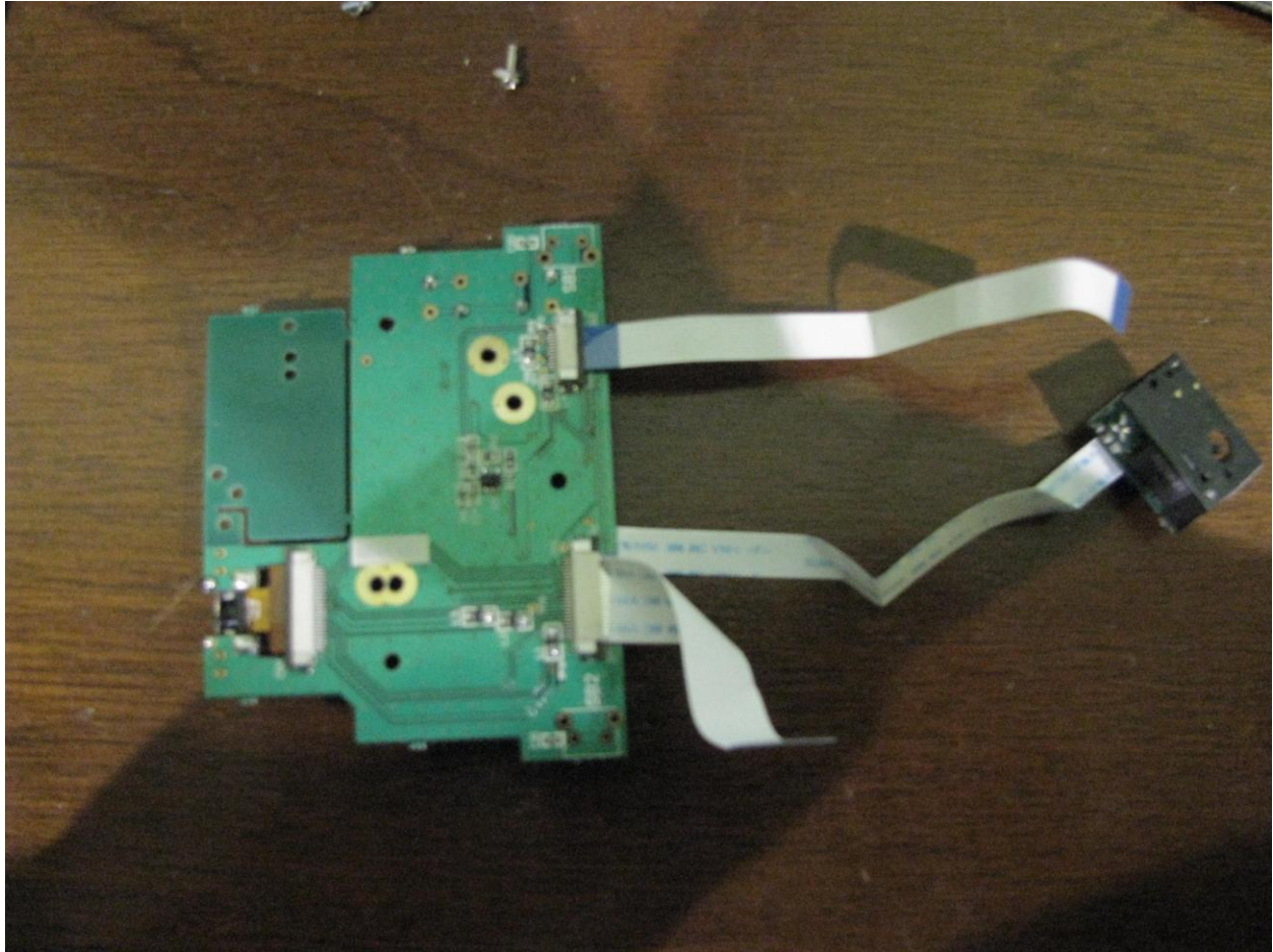
Figure 9: IR Port PCB (Placed on top cover of EUT) Bottom side
