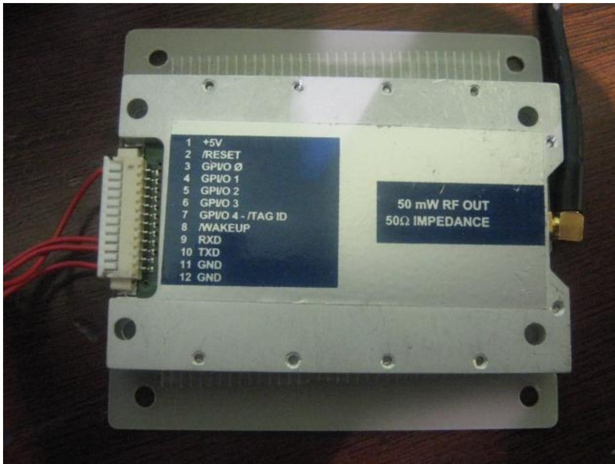
Figure 1 – RF Chip
