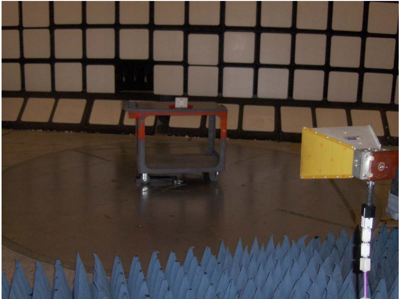
Radiated Emissions at 3m Distance Orthogonal Position 2
