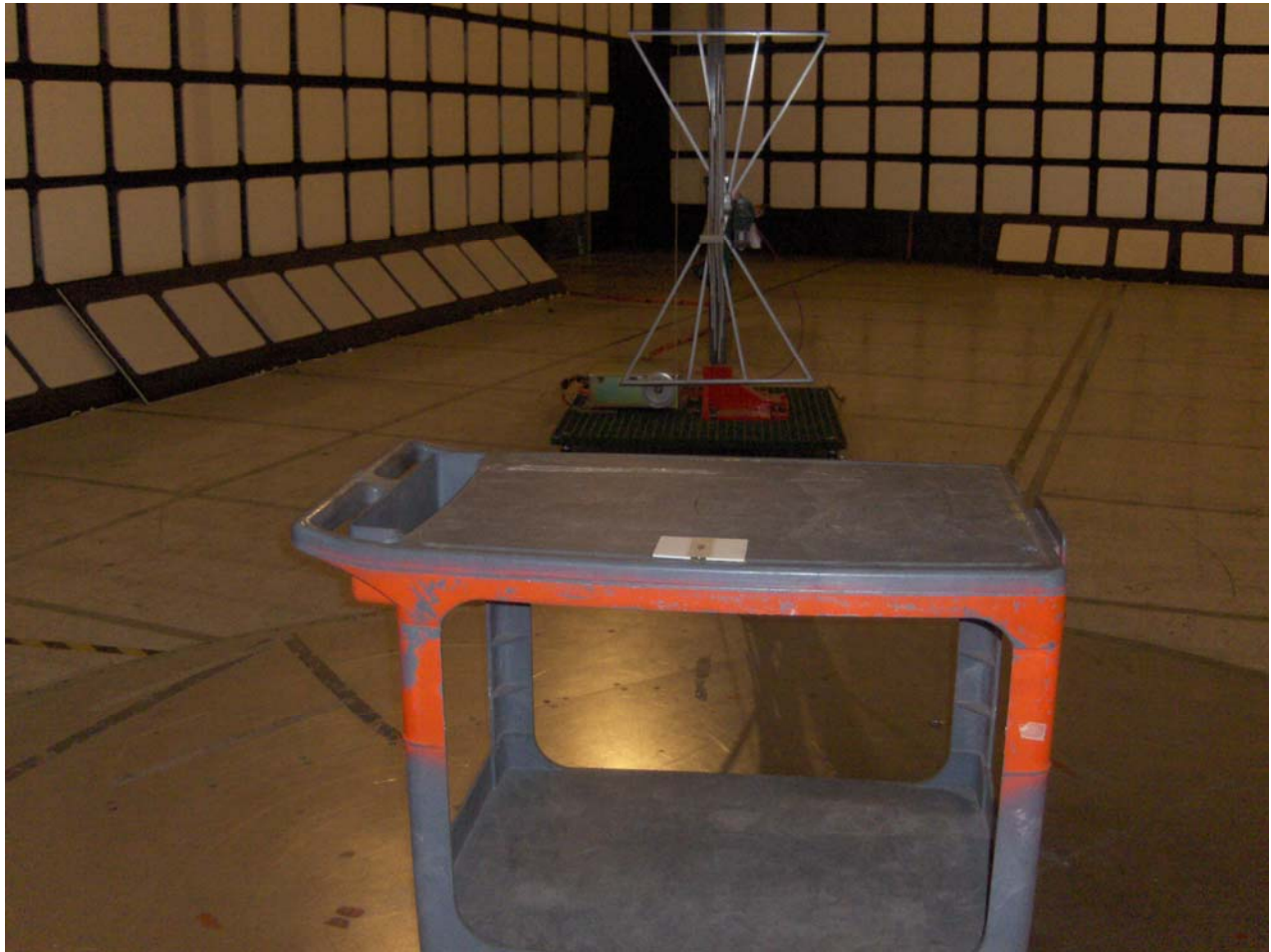
Radiated Emissions at 3m Distance Orthogonal Position 1
