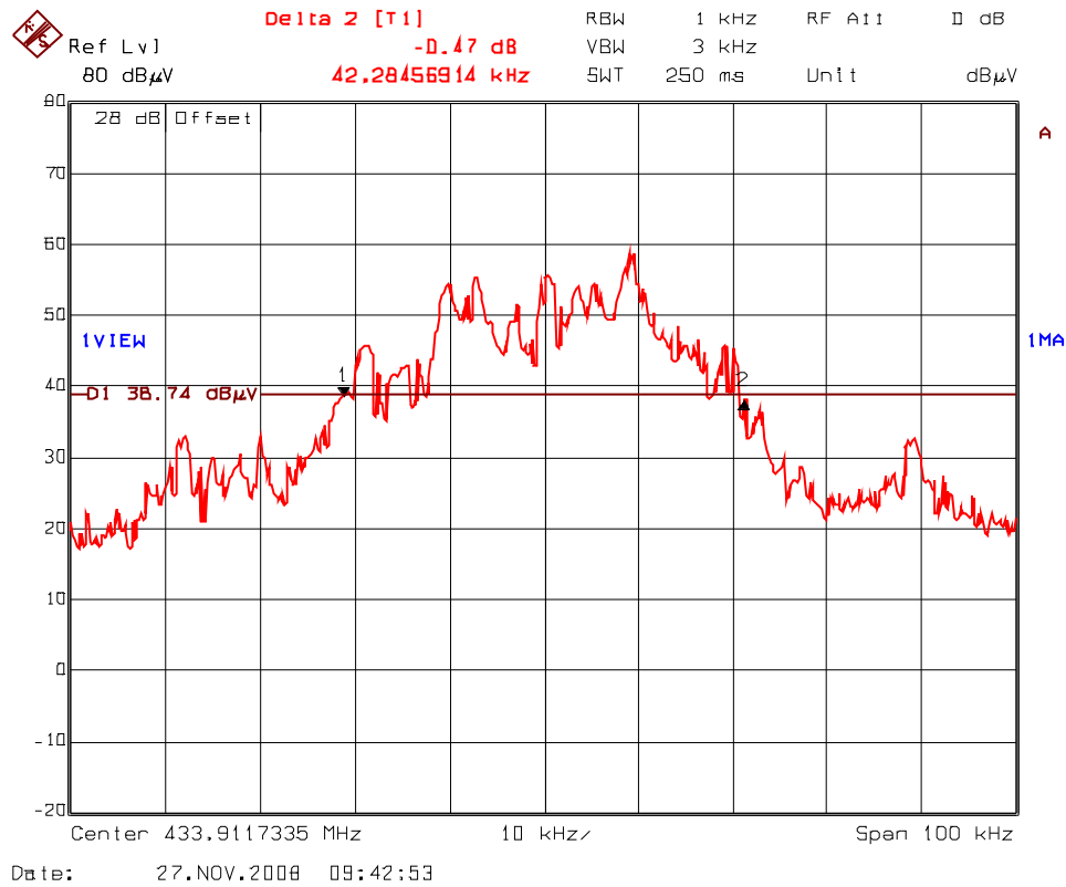
Plot 5.7.3.1: 20 dB Bandwidth Fc: 433.92 MHz
