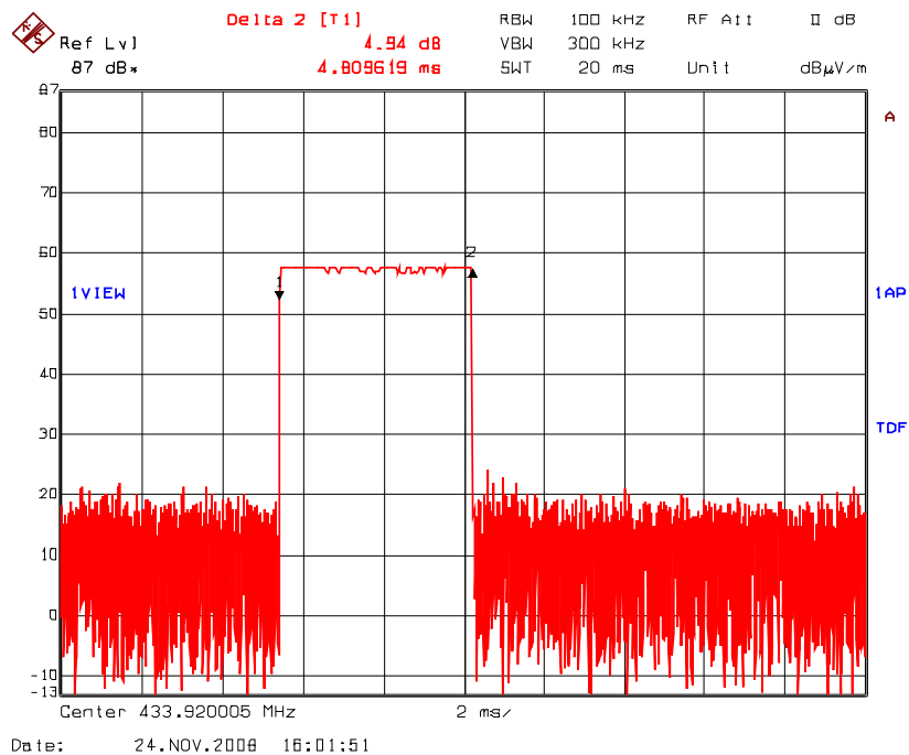
Plot 5.6.3.1(ii) Duty Cycle (pulse length is 4.81 ms)
