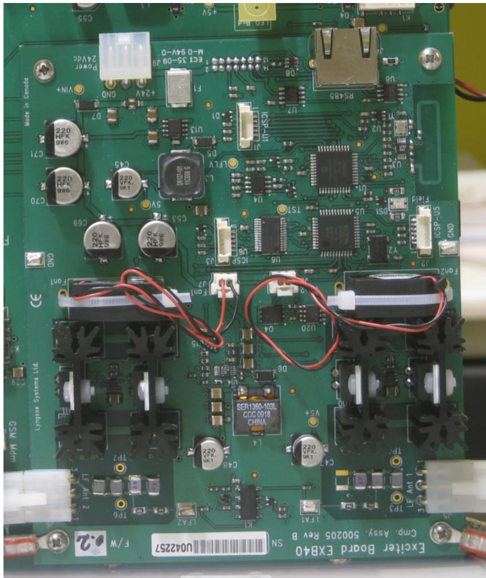
Exciter Board (EXB40) Top
