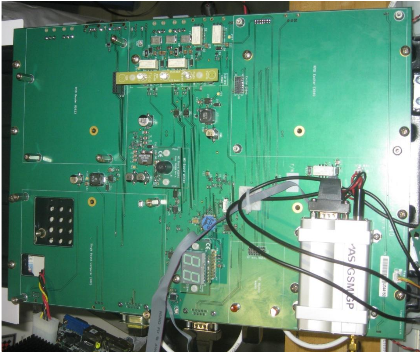
Reverse side of main board (populated without daughter cards)
