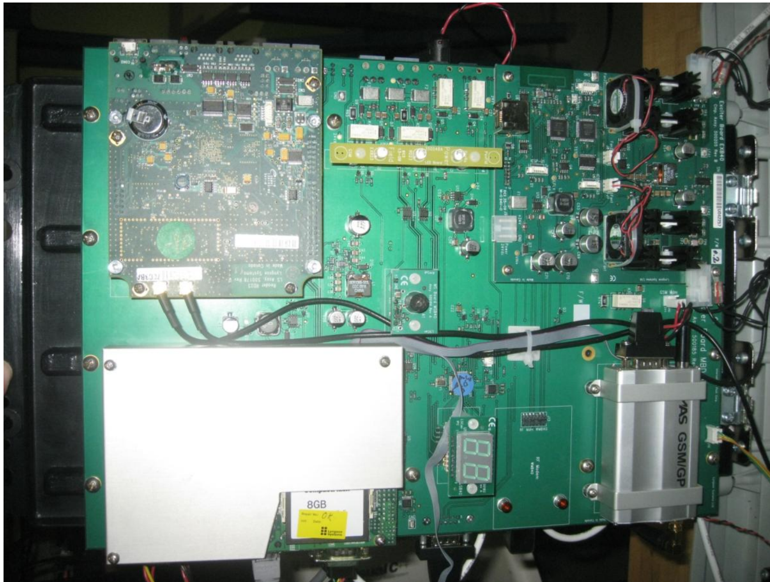
Reverse side of main board (populated with daughter cards)
