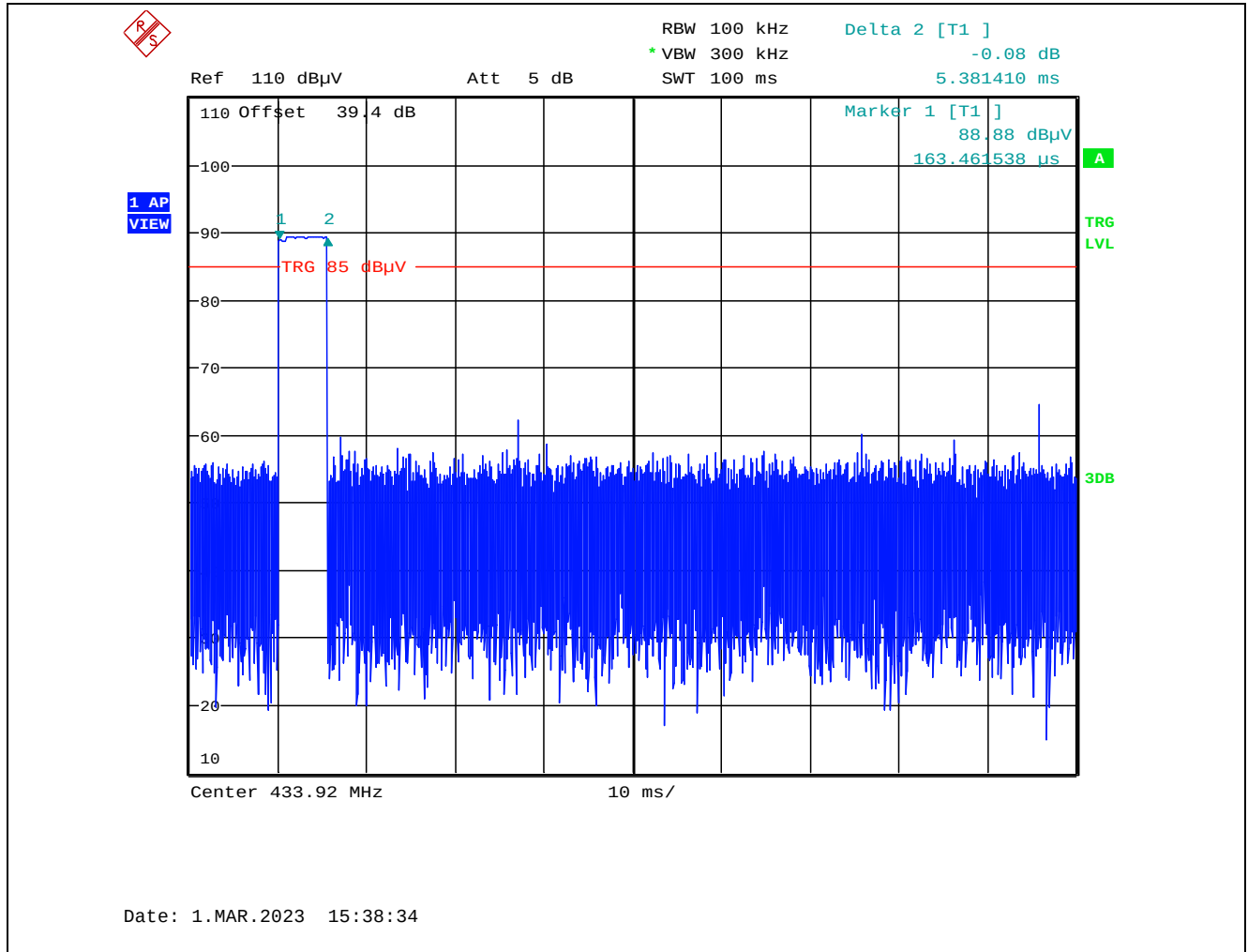
Plot 5.2.3.3.2. Duty Cycle (100 ms)
