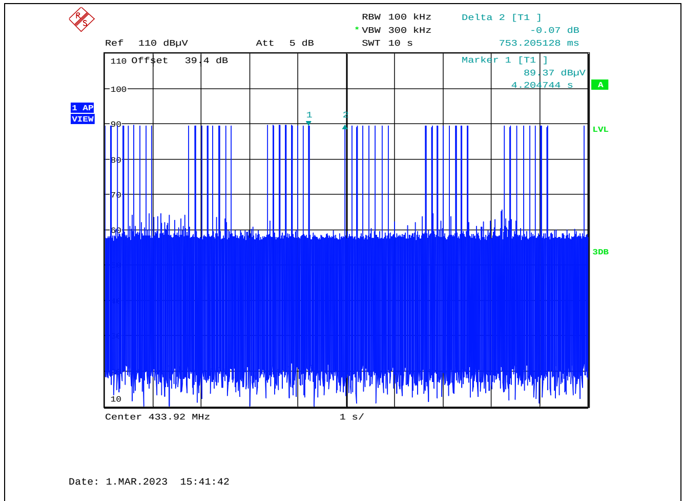
Plot 5.2.3.3.1. Duty Cycle (Pulse Train)
