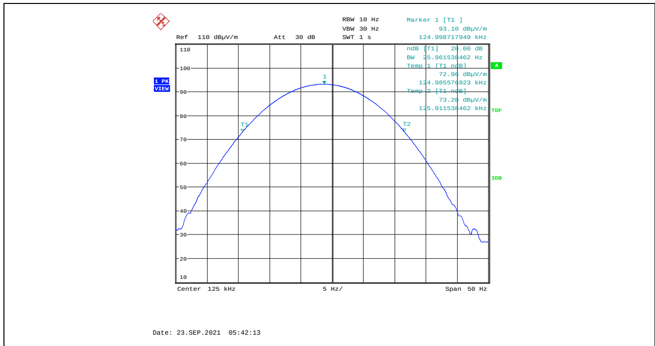
Plot 5.3.3.1. 20 dB Bandwidth, Fc: 125 kHz Command SM1, Modulation Constant to "1" (SM1)
