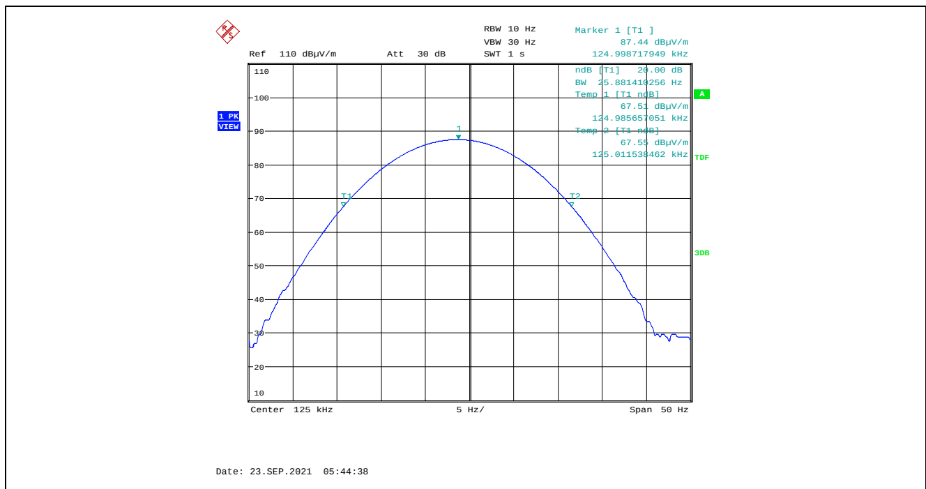
Plot 5.3.3.2. 20 dB Bandwidth, Fc: 125 kHz Command SM2, OOK Modulation with 600 Hz (SM2)
