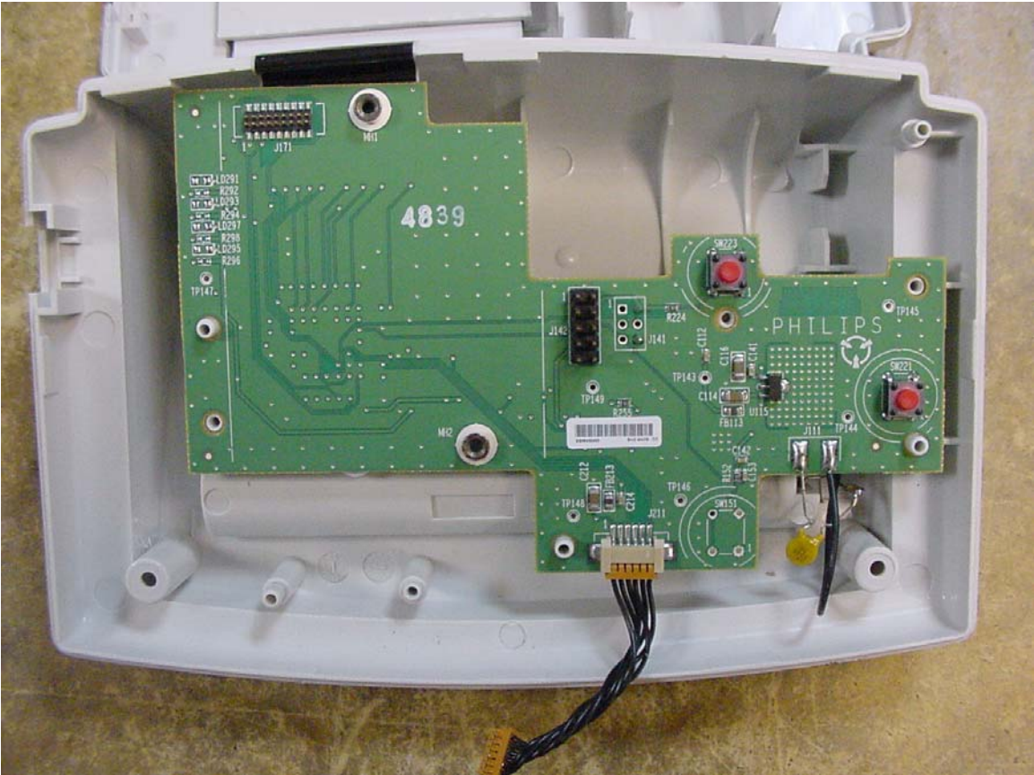
Internal, Inside, front board
