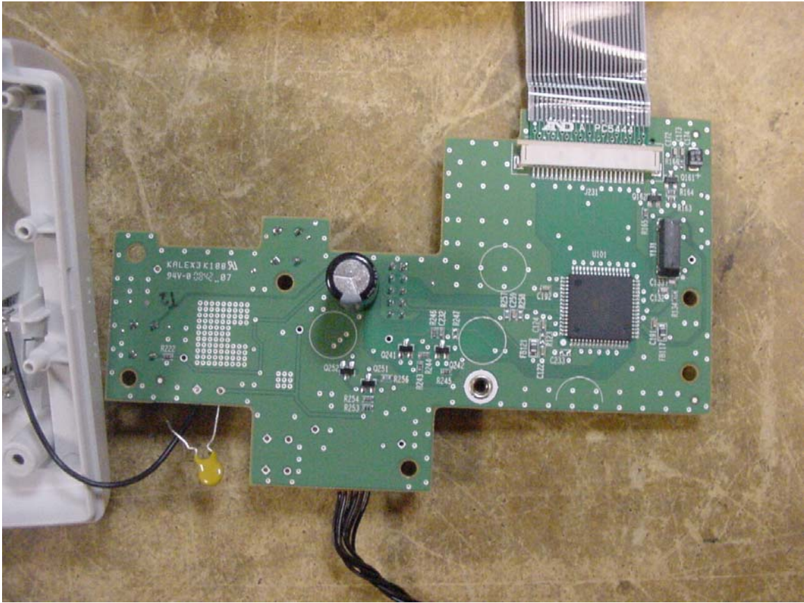
Internal, Rear of board
