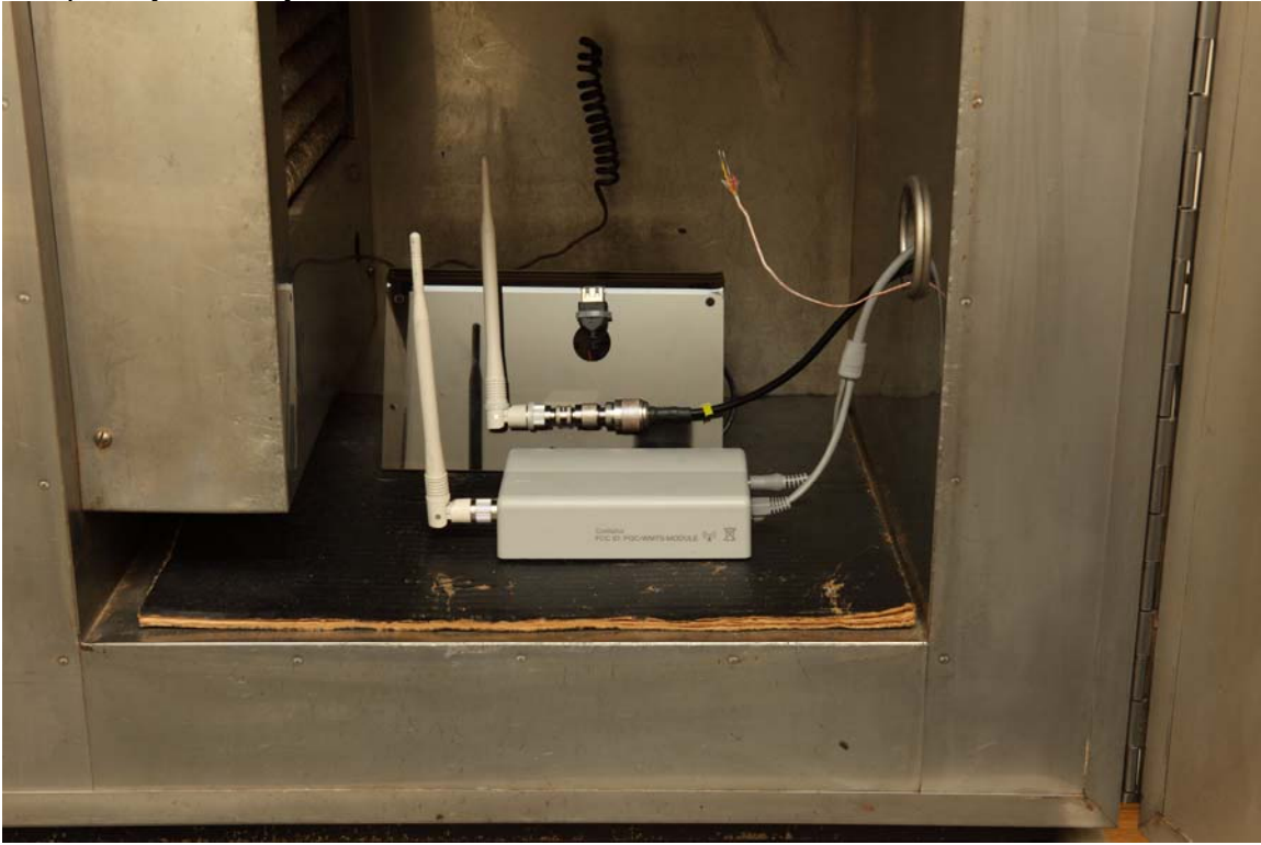
Frequency Stability
