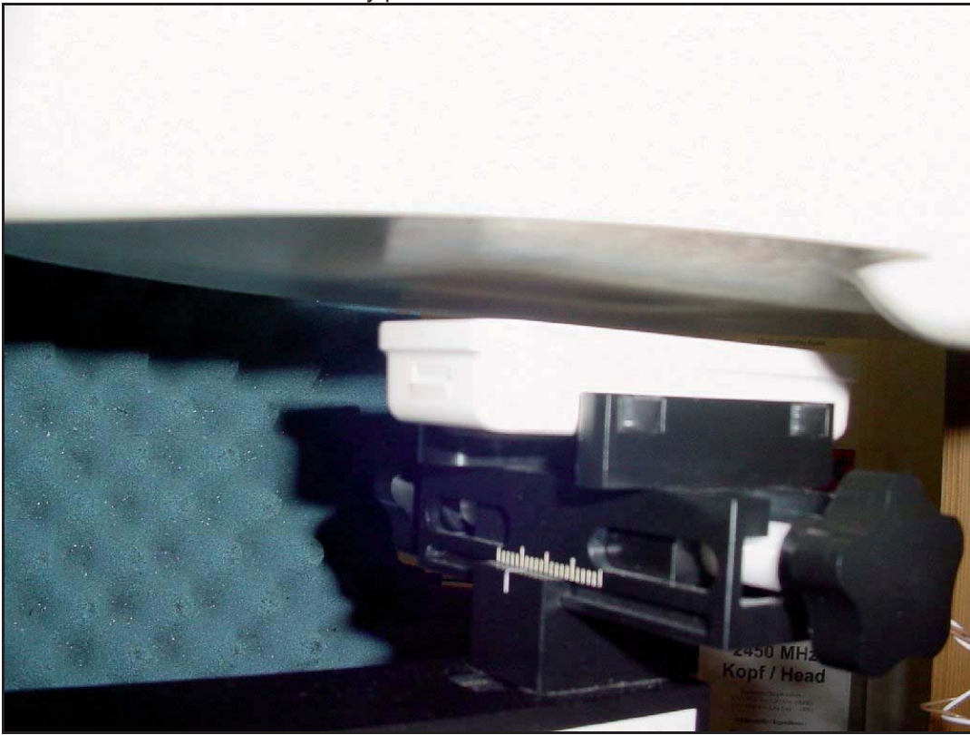
Photo 6: Test body position rear side without any distance
