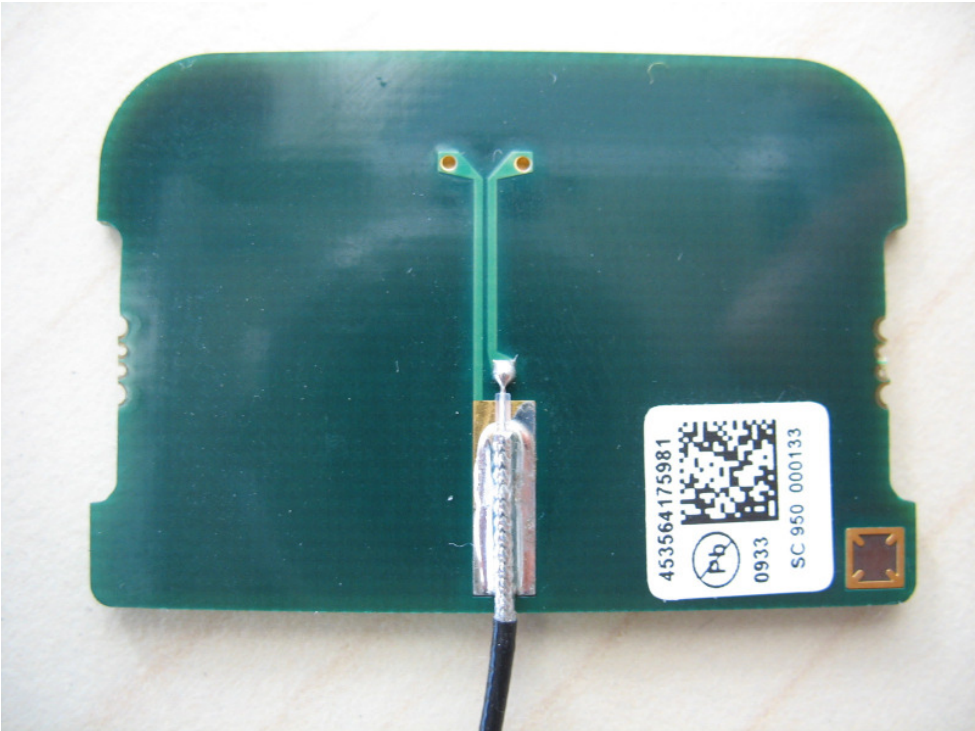
Photo 6: (Antenna)
