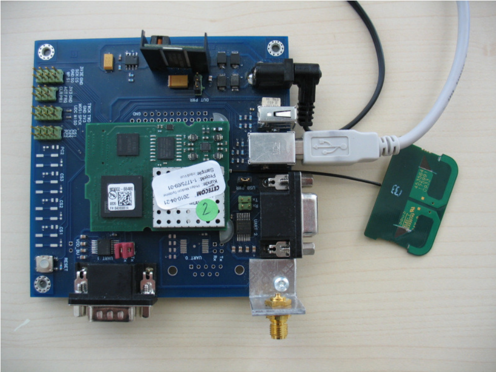
Photo 1 (Test board / WLAN Module / Antenna):
