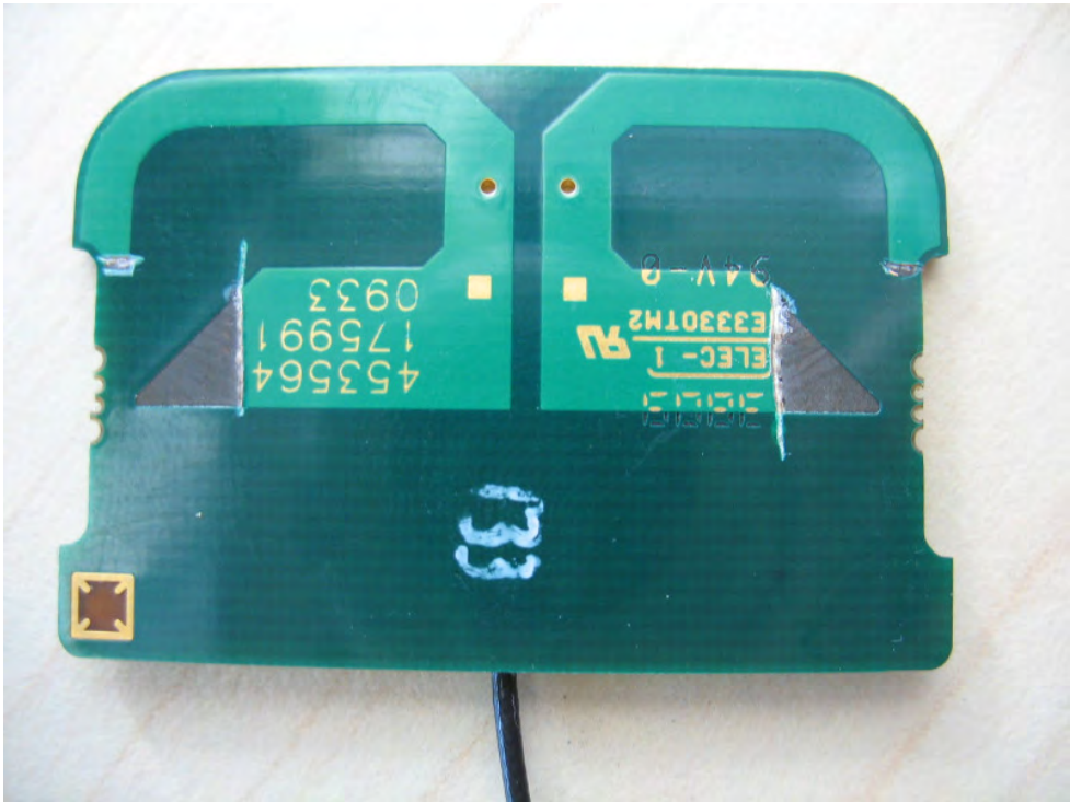
Photo 7: (Antenna)
