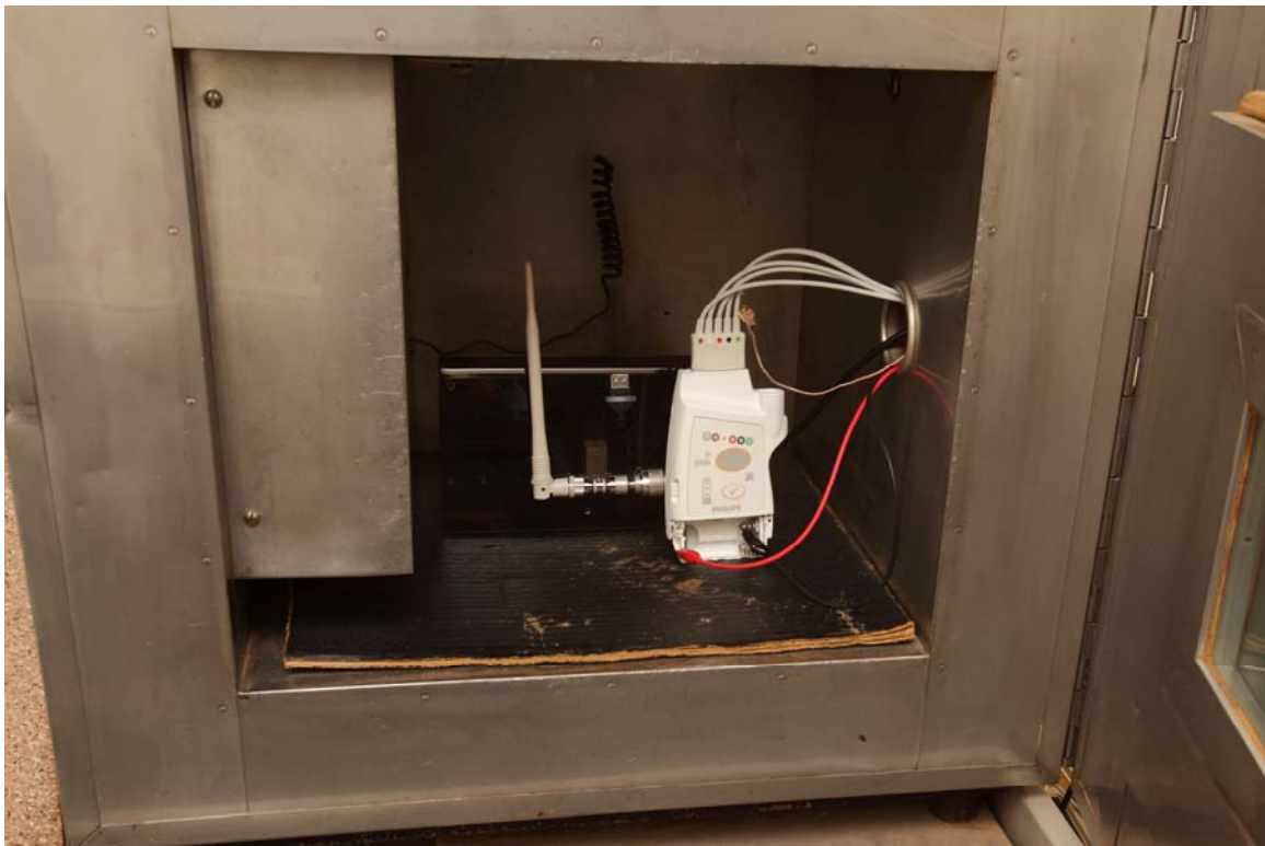
Frequency Stability
