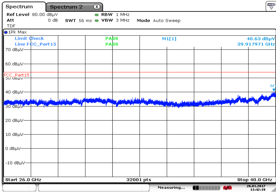
Plot 54: 26 GHz to 40 GHz, 5795 MHz, vertical & horizontal polarization
