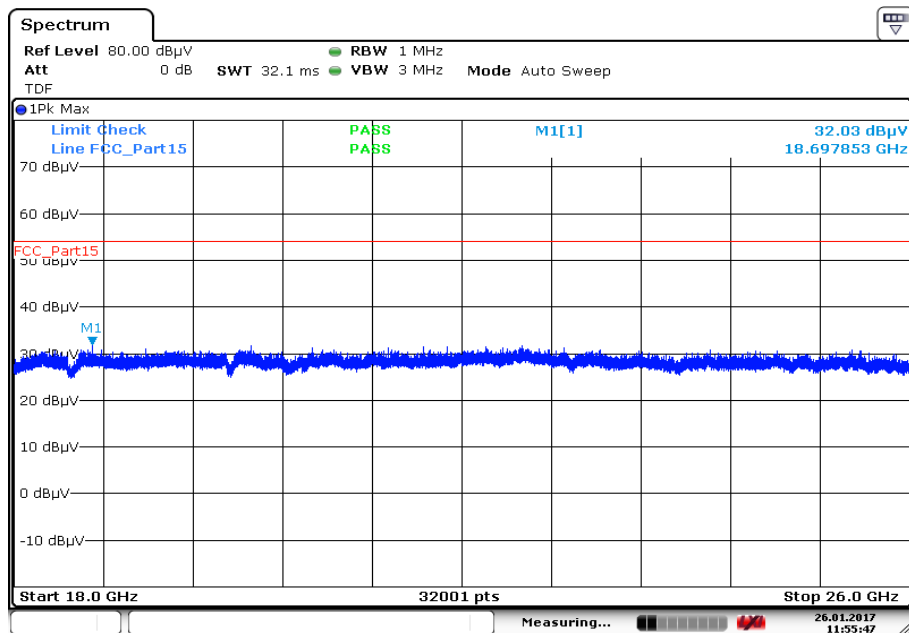
Plot 35: 18 GHz to 26 GHz, 5600 MHz, vertical & horizontal polarization
