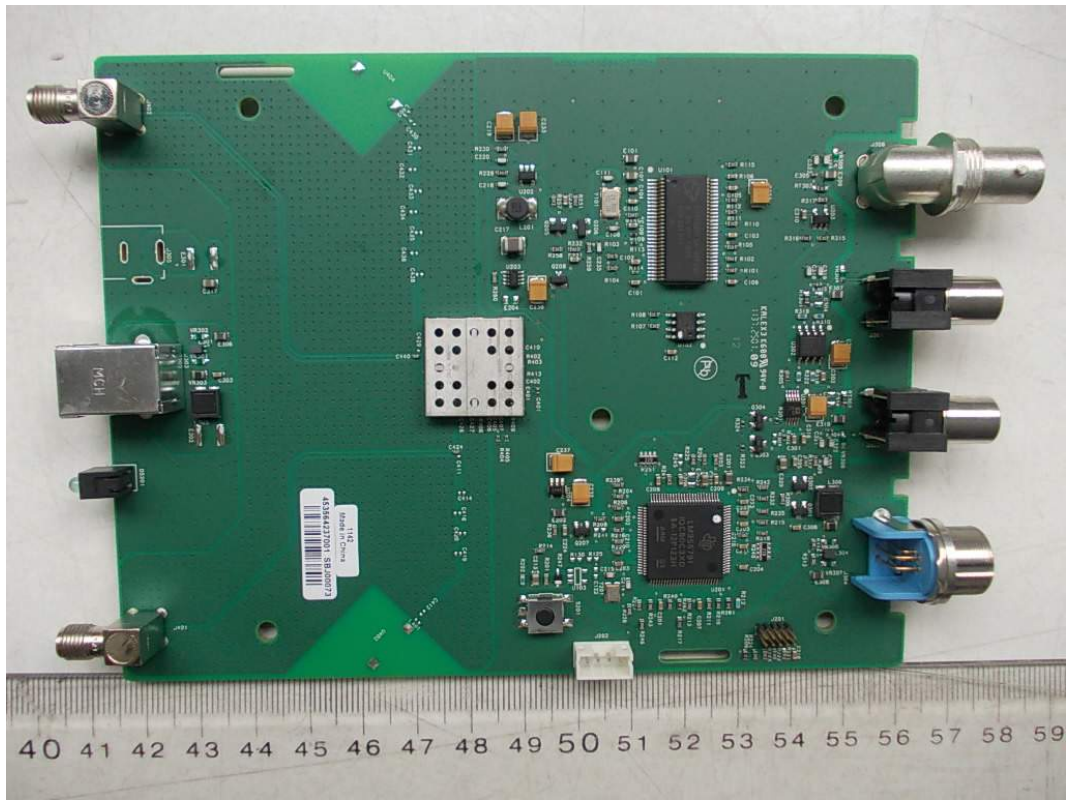
FIGURE 2 ADVANCED INTERFACE MODULE (M/N: ST80i AIM) MAIN BOARD (FRONT VIEW)
