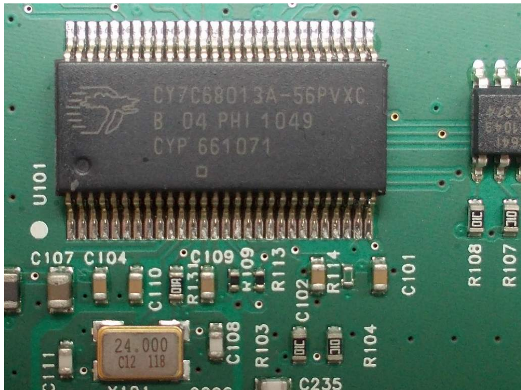
FIGURE 4 ADVANCED INTERFACE MODULE (M/N: ST801 AIM) CHIP & CRYSTAL #1 ON MAIN BOARD
