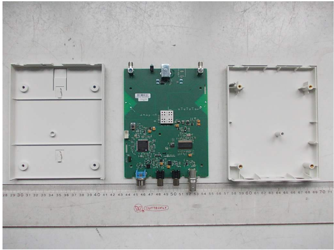
FIGURE 1 ADVANCED INTERFACE MODULE (M/N: ST801AIM) COVER REMOVED
