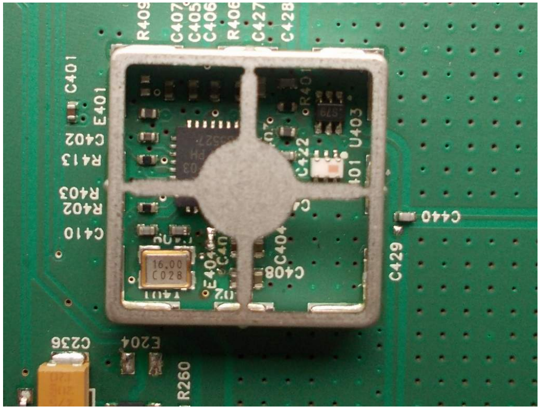
FIGURE 6 ADVANCED INTERFACE MODULE (M/N: ST801 AIM) RF MODULE ON MAIN BOARD
