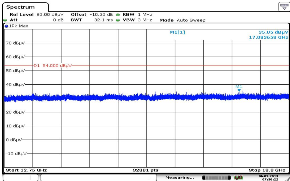
Plot 7: Middle channel, 12 GHz to 18 GHz, vertical & horizontal polarization
