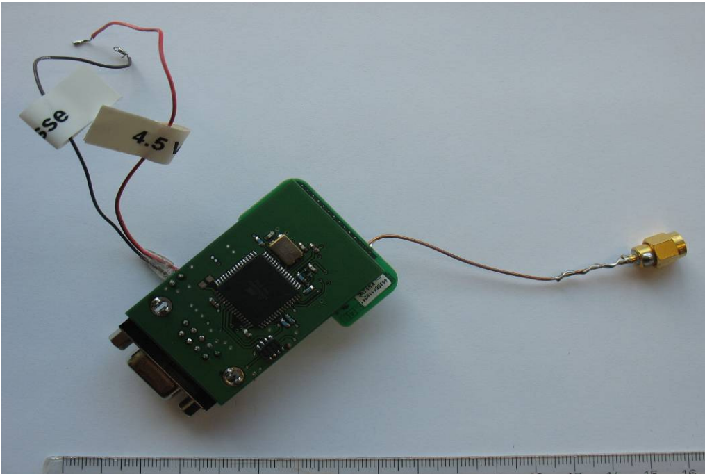
Photo 2: conducted test sample mounted on test board
