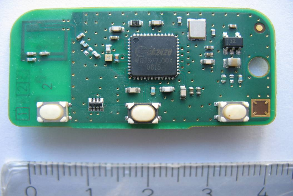
Photo 7: Radiated sample
