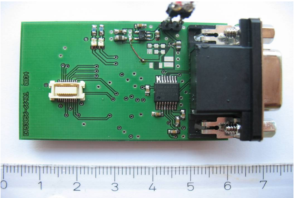
Photo 4: test board
