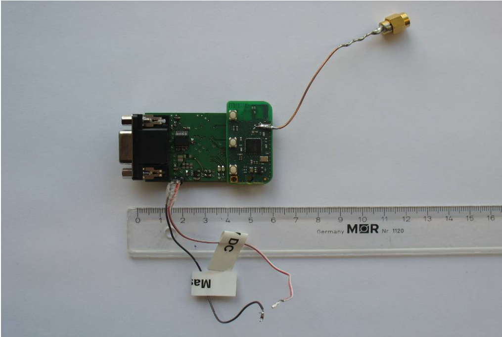
Photo 1: conducted test sample mounted on test board
