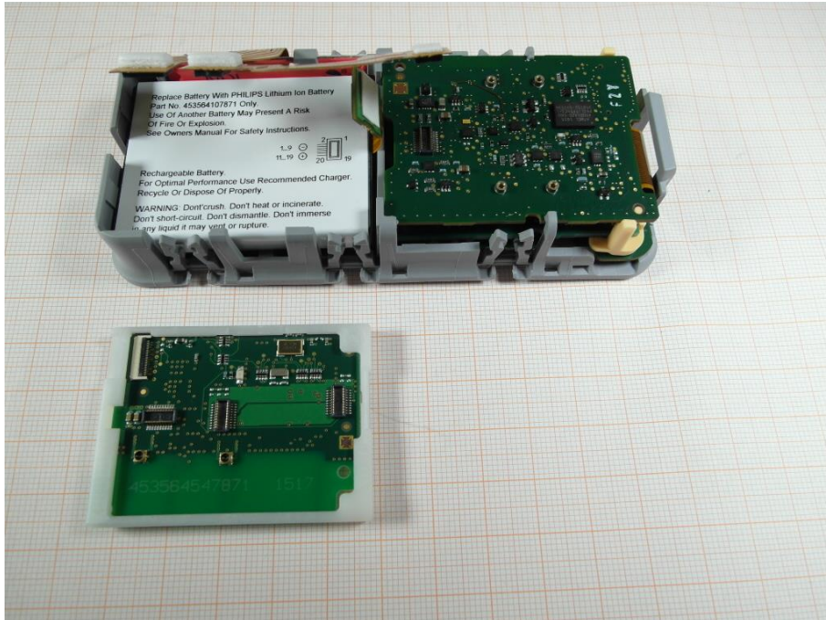
Photo 3: PCB 1 removed
