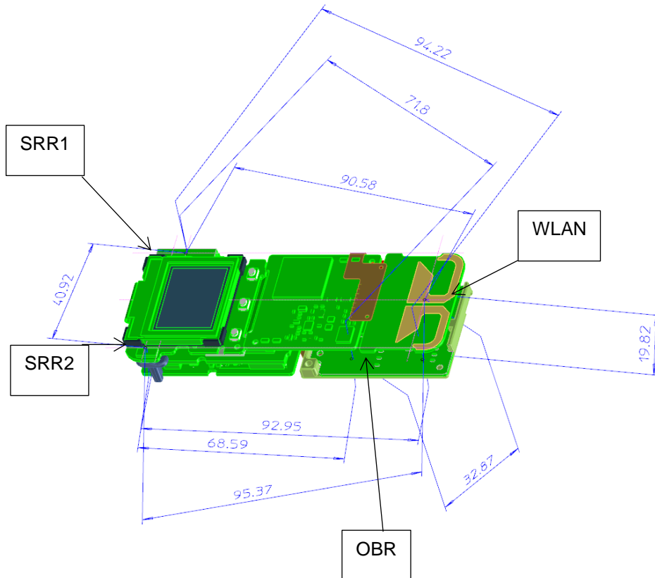
Photo 10: Antenna dimensions and separation distances
