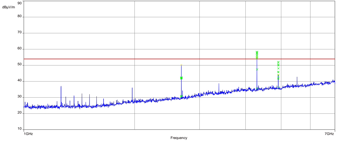
Plot 9: 1 GHz – 7GHz, mid channel
