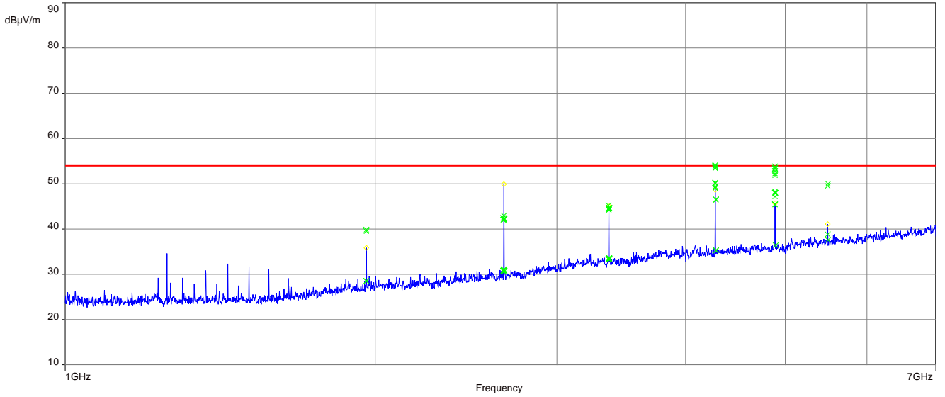
Plot 6: 1 GHz – 7GHz, mid channel
