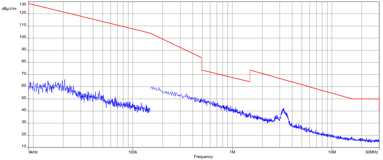
Plot 4: 9 kHz – 30 MHz, mid channel
