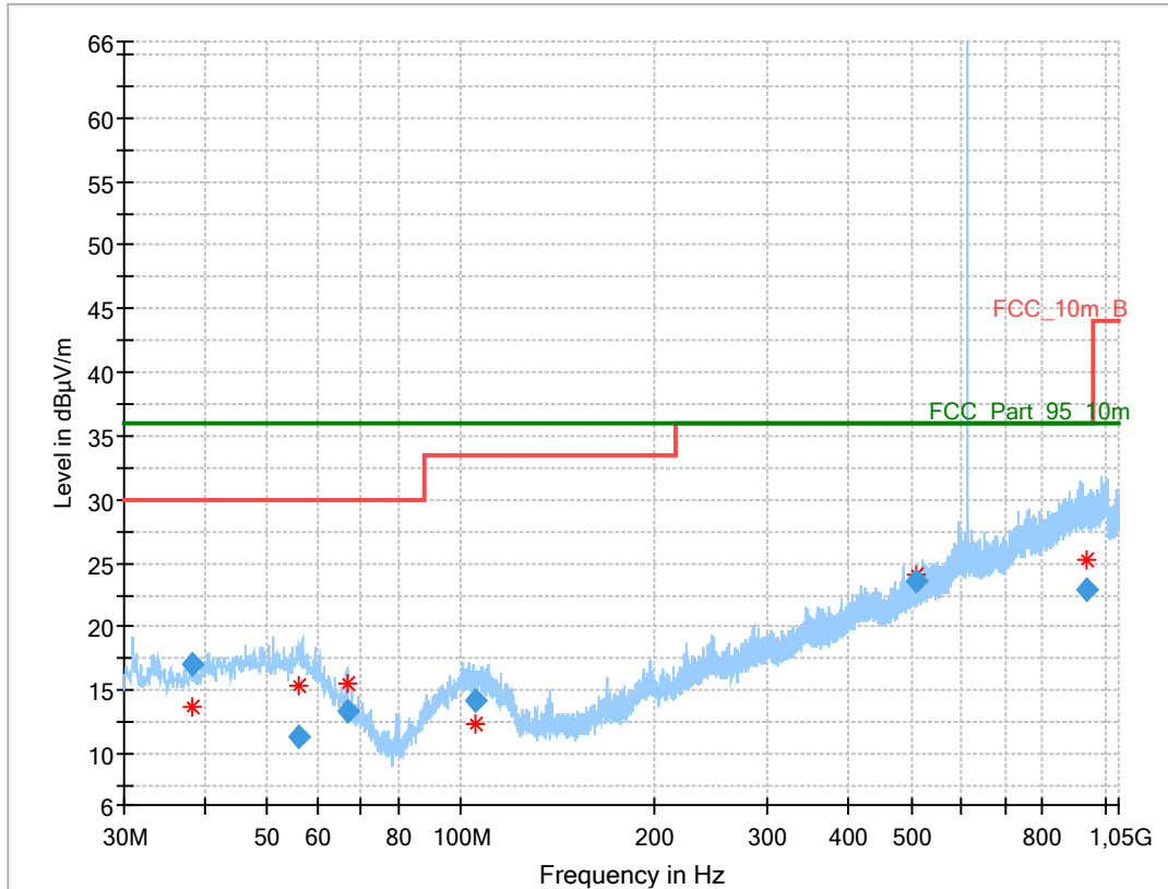
Plot 5: 30 MHz – 1 GHz, mid channel
